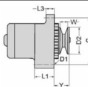
type B 2-bolt fixing
