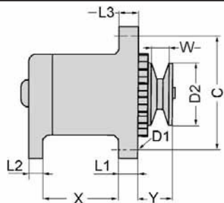
type A 3-bolt fixing
